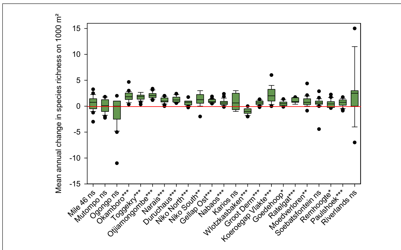
Fig. 8: Mean annual changes in species richness of the major perennial life forms phanerophytes and chamaephytes on 1000-m 2 plots over the observed period (2–9 years). The graphs depict medians (lines), inter-quartile ranges (boxes), inter-decile ranges (hinges), and extreme values (dots). The symbols after the Observatory names denote the significance of richness changes: ns: p \geq 0.05 ; *: p < 0.05 ; **: p < 0.01 ; ***: p < 0.001 .
